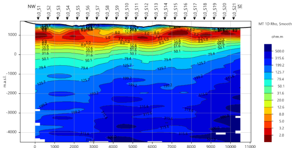
Figure 1. Tonopah Lithium Project – MT survey data
