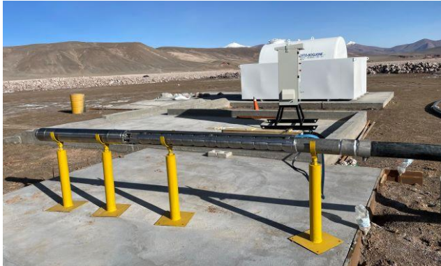
Figures 3-4. Rincon Lithium Project – 2,000tpa Operation Brine Systems Site Works
